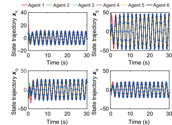
Fig. 2 State trajectories of the multi-agent system under PD control ( i = 1, 2, \dots, 6 ) (References to color refer to the online version of this figure)
