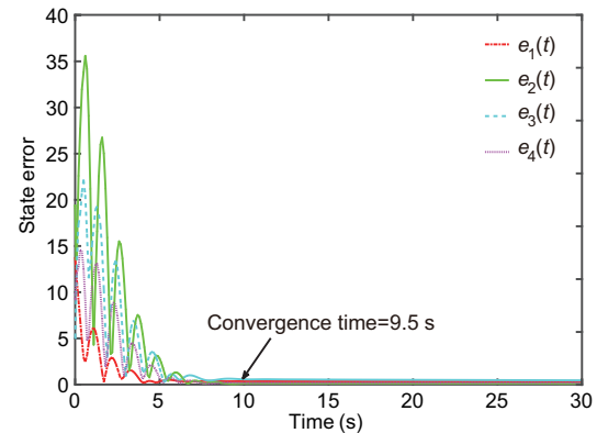
Fig. 5 State errors of the multi-agent system under PID control
